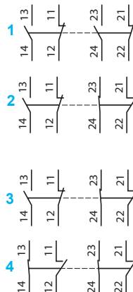
Example: contact schematics of XMLD
